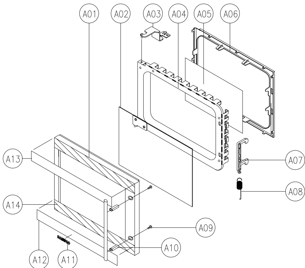
DOOR ASSEMBLY KOR-634R0S:3511712140
