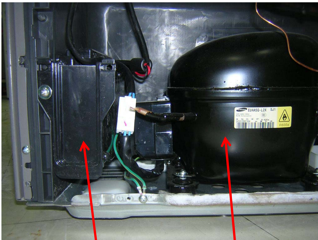
INVERTER BOX
