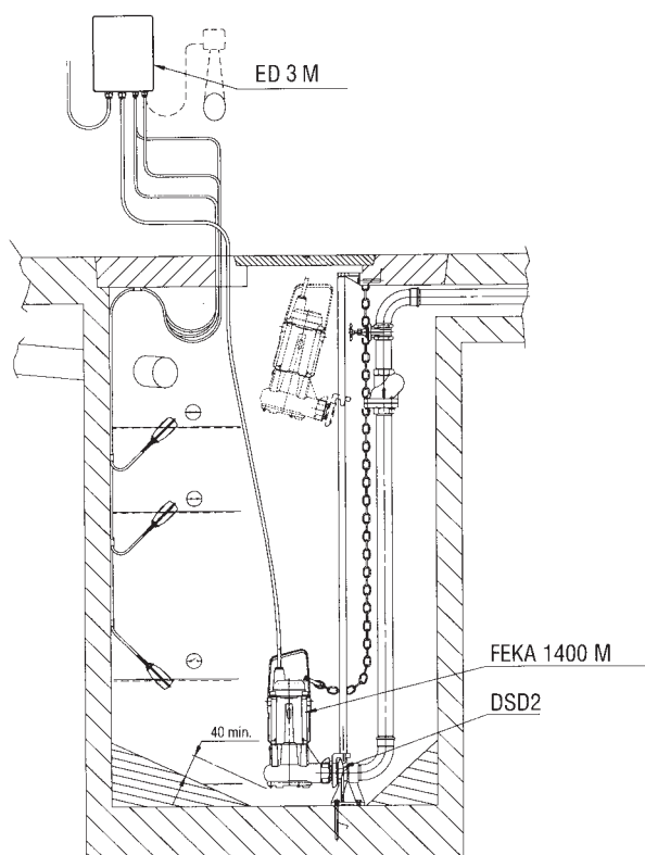
Fixed installation with 1 Feka 1400 M pump with DSD2 device, complete with ED 3 M control unit, with two minimum and maximum level control floats and one alarm float.
