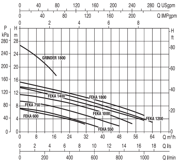
Curves refer to two pumps in function.
