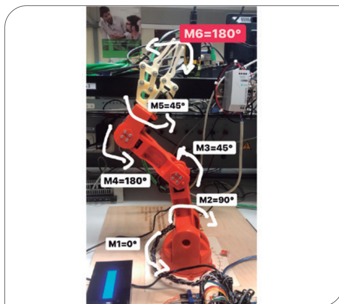
Figure 1 Robotic Manipulator [2] (braccio-robot).
