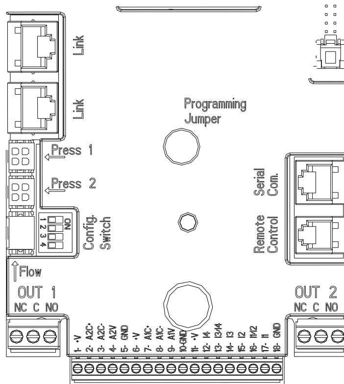
Figure 3: Connections
