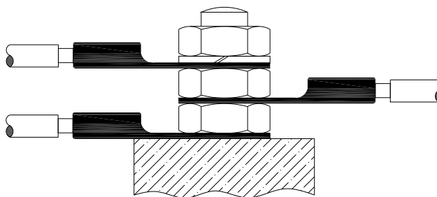
Figure 2: Earth connection
