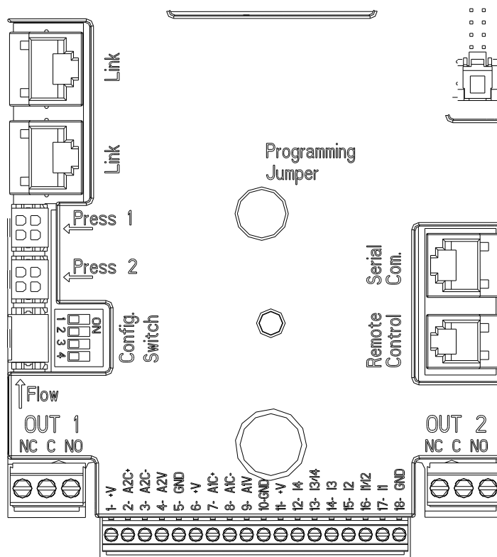
Figure 3: Connexions
