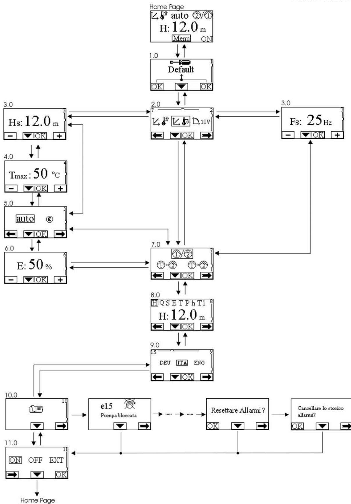
Figure 8: MCE Menu
