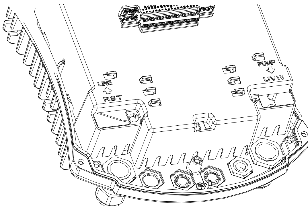
Figure 1: Electrical connections
