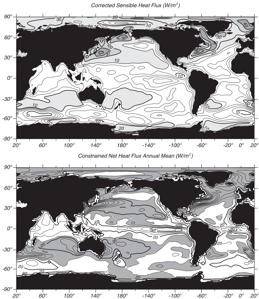
Figure 5.10 Annual-mean upward sensible heat flux Q_S ( top ) and constrained, net, downward heat flux ( bottom ) through the sea surface in \text{W}/\text{m}^2 calculated by DaSilva, Young, and Levitus (1995) using the ICOADS data set from 1945 to 1989. Contour interval is 2 \text{ W}/\text{m}^2 (top) and 20 \text{ W}/\text{m}^2 (bottom).
