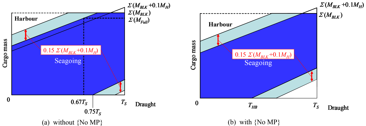
Fig. 5 Example of mass curve for BC-A ships with “Block loading”
