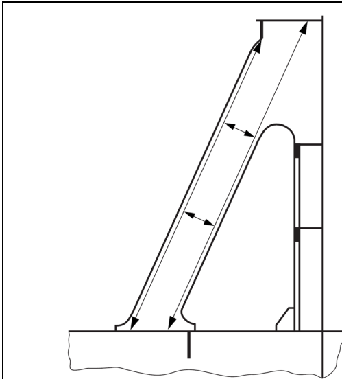
Fig. 4 Coaming stay: example 3
