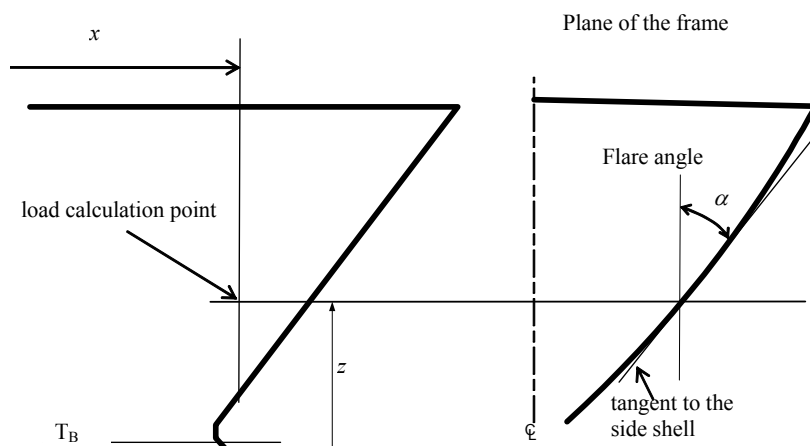
Fig. 6 The definition of the flare angle
