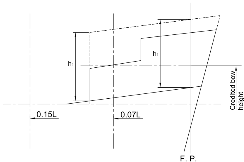
Fig. 2 Credited bow height where the freeboard deck has shear extending for less than 0.15L
