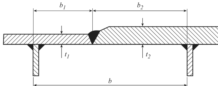
Fig. 1 Plate thickness change within the field breadth
