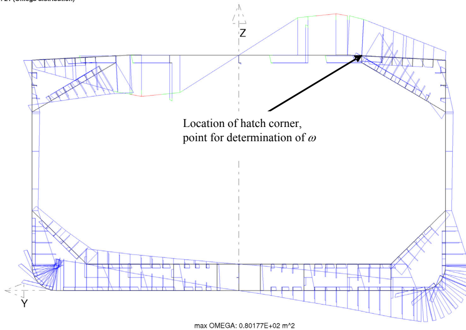
Fig. 1 Cross section for determination of I_T and \omega
