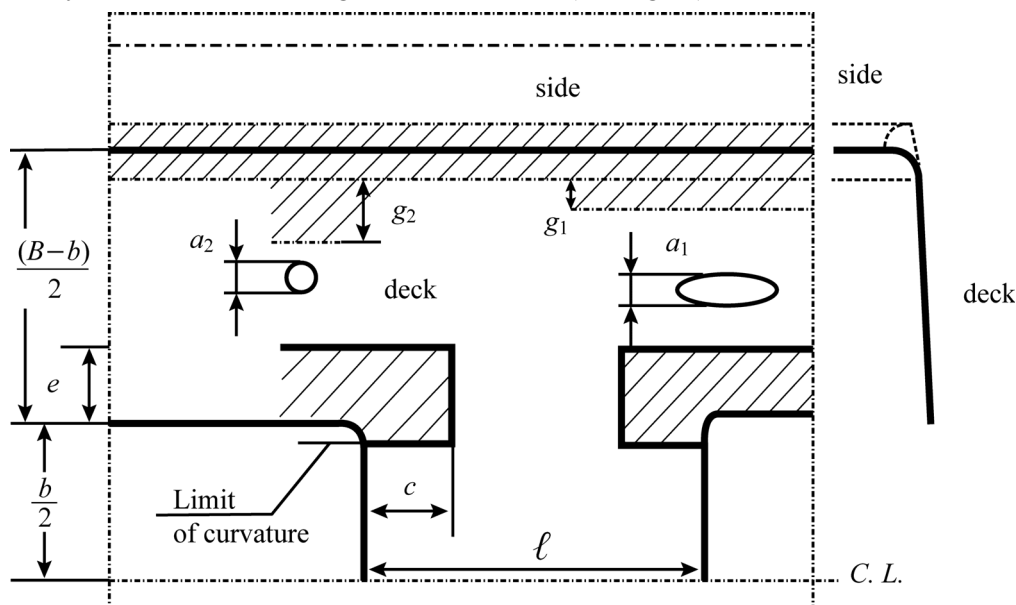
Fig. 23 Position of openings in strength deck
