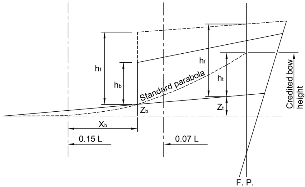
Fig. 1 Credited bow height where the freeboard deck has shear extending from abaft 0.15L
