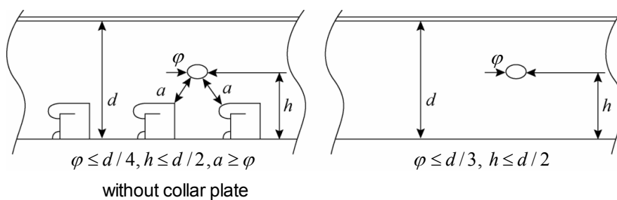
Fig. 15 Location and dimensions of lightening holes
