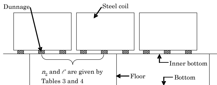
Fig. 3 Loading condition of steel coils (Example of n_2 = 4, n_3 = 3 )
