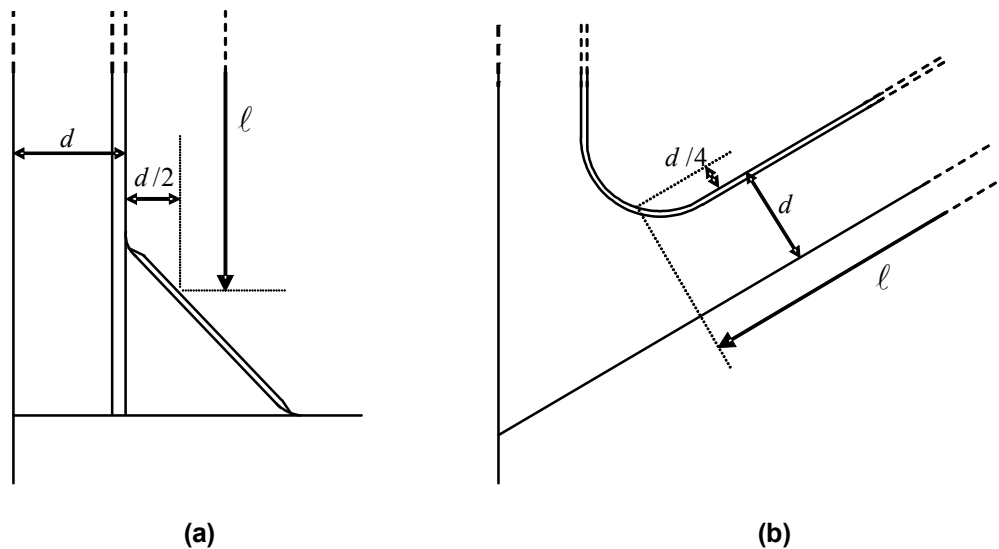
Fig. 13 Span of primary support member
