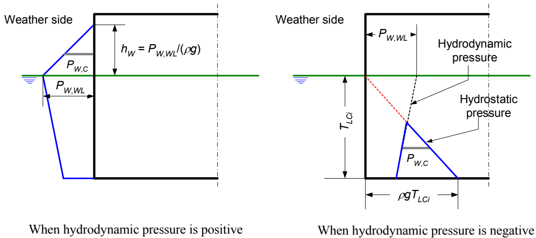
Fig. 5 Correction to hydrodynamic pressure
