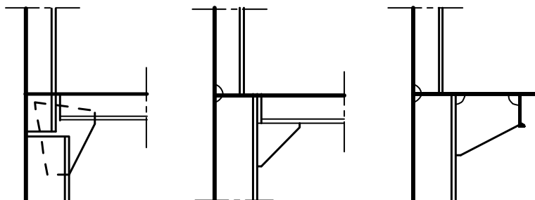
Fig. 1 End attachment of superstructure frames
