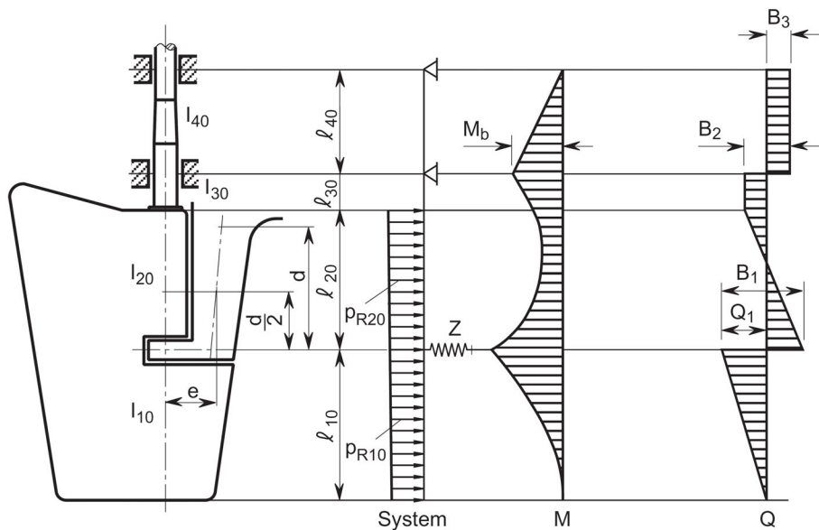
Fig. 4 Semi-spade rudder (with 1-elastic support)
