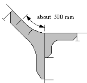
Fig. 7 Example of insertion of horizontal gusset or longitudinal rib
