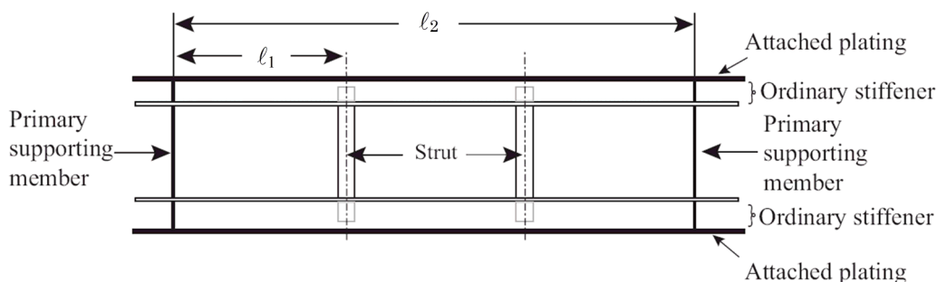
Fig. 5 Span of ordinary stiffeners with two struts
