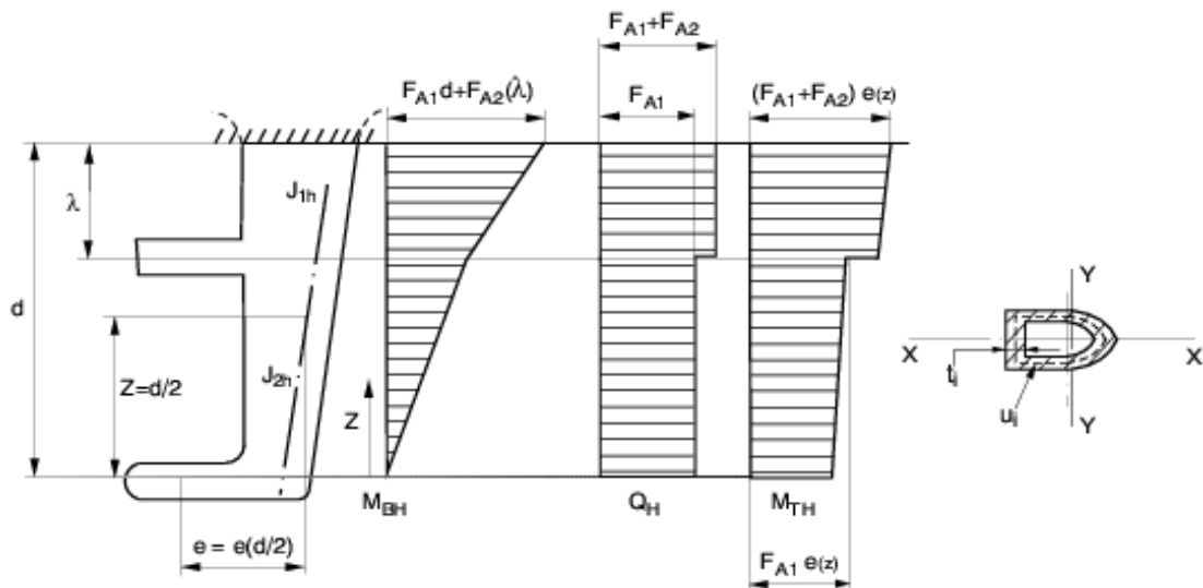
Fig. 19 Geometry of rudder horn
