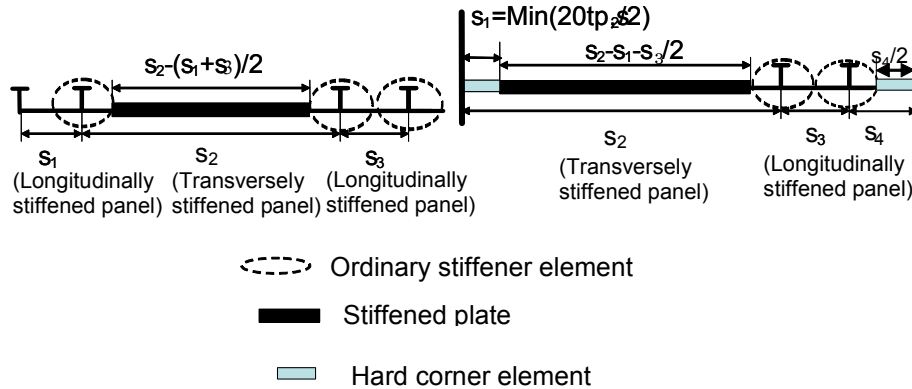
Fig. 2 Extension of the breadth of the attached plating and hard corner element
