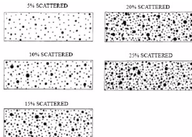
Fig. 6 Pitting intensity diagrams (from 5% to 25% intensity)
