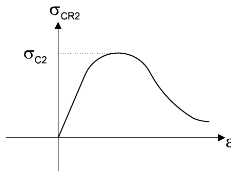
Fig. 9 Load-end shortening curve \sigma_{CR2}-\varepsilon for flexural-torsional buckling
