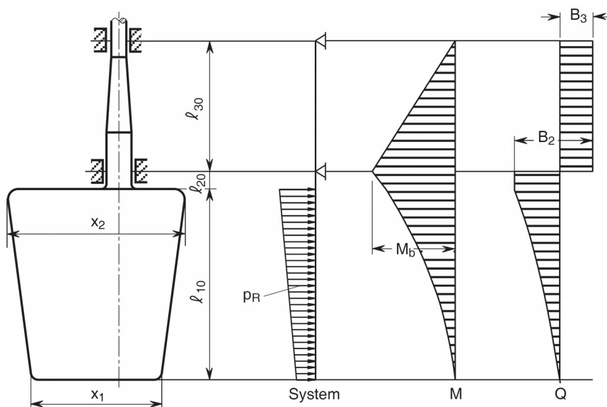
Fig. 5 Semi-spade rudder (with 2-conjugate elastic supports)
