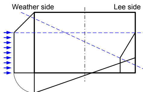
Fig. 3 Distribution of hydrodynamic pressure p_{R1} at midship
