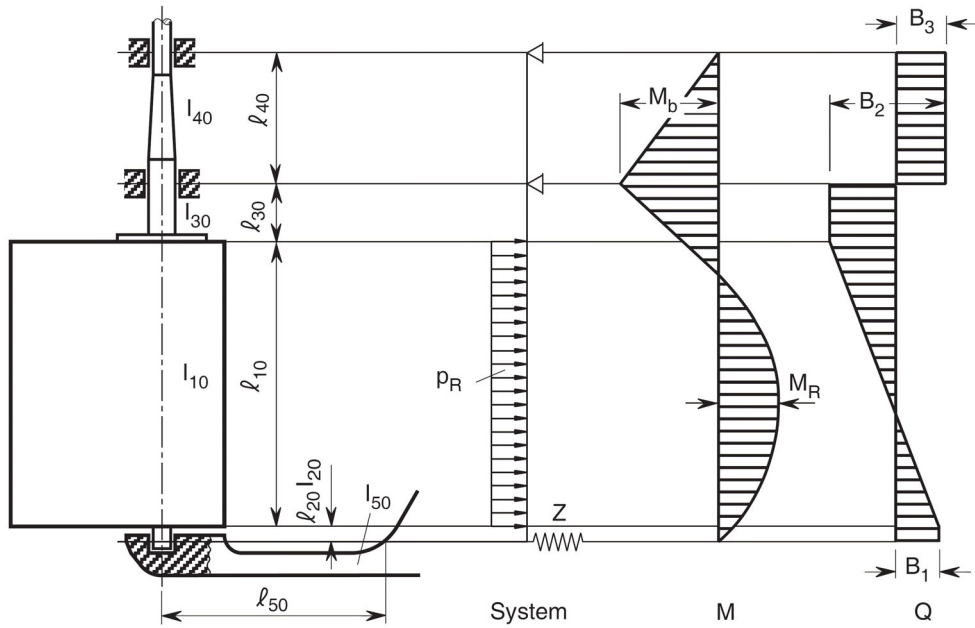
Fig. 3 Rudder supported by sole piece
