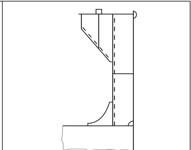
Fig. 3 Coaming stay: example 2
