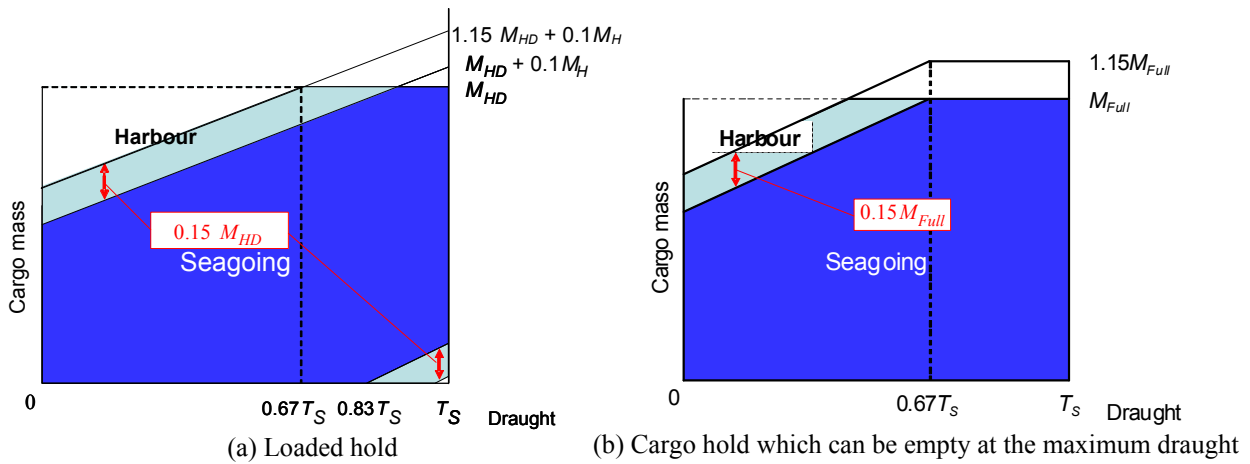
Fig. 1 Example of mass curve for BC-A ships not having {No MP} assigned
