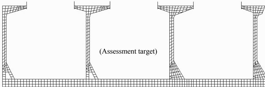
Fig. 1 Longitudinal extent of the finite element model
