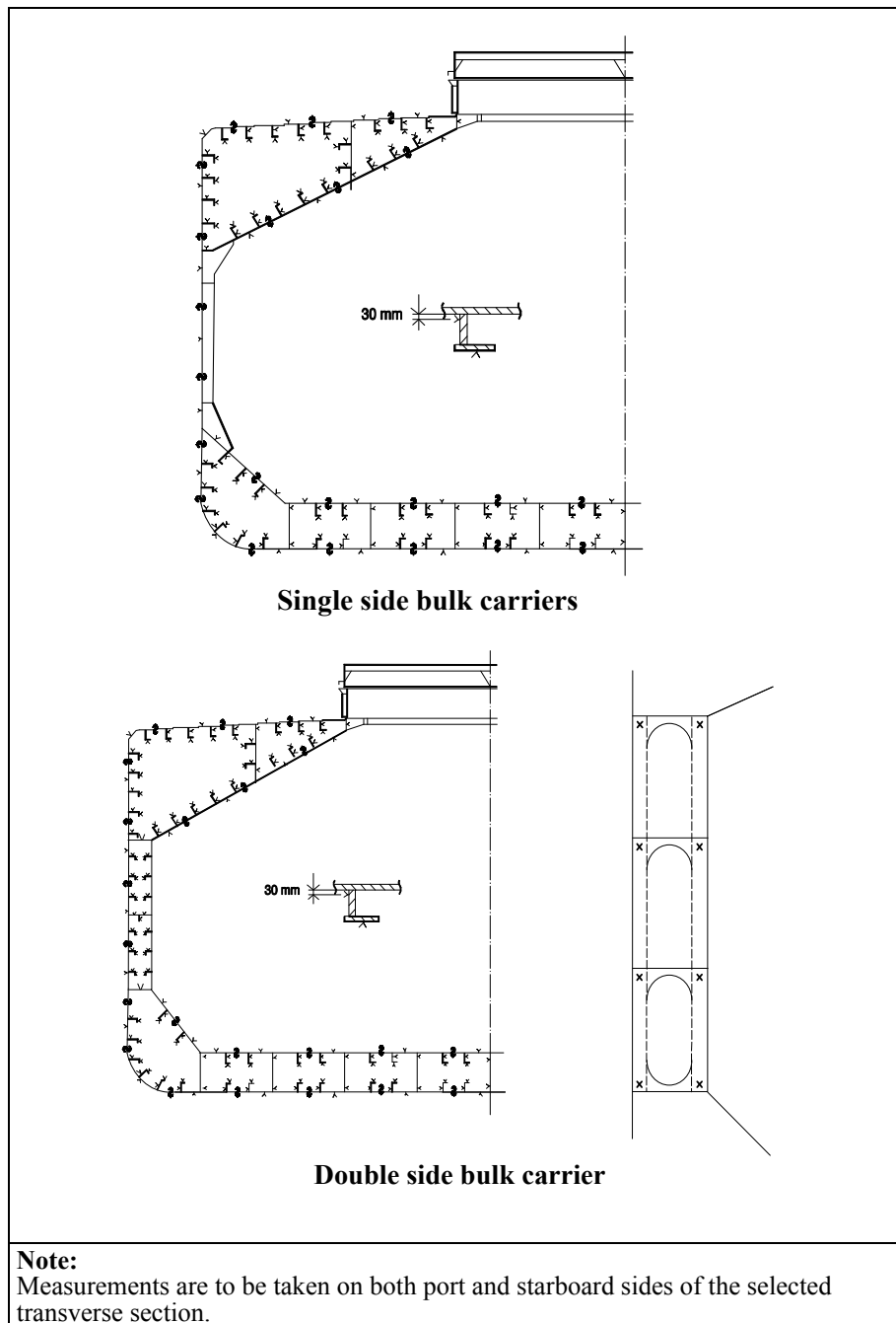
Fig. 1 Transverse section of bulk carrier
