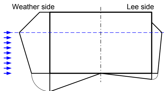
Fig. 4 Distribution of hydrodynamic pressure p_{P1} at midship
