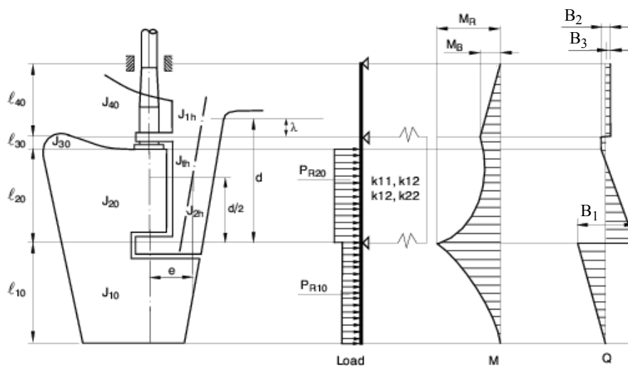
Fig. 5 Semi-spade rudder (with 2-conjugate elastic supports)
