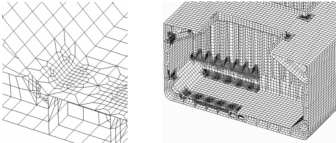
Fig. 1 “Direct” modelling with refined meshes
