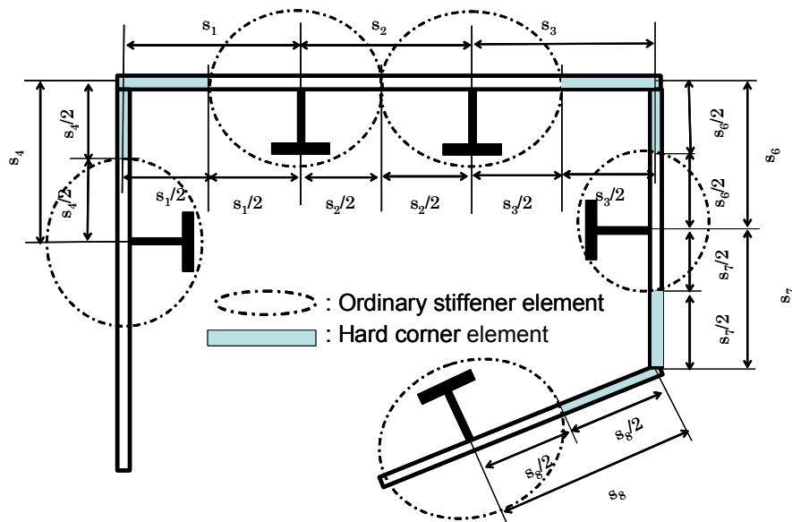
Fig. 3 Extension of the breadth of the attached plating and hard corner element
