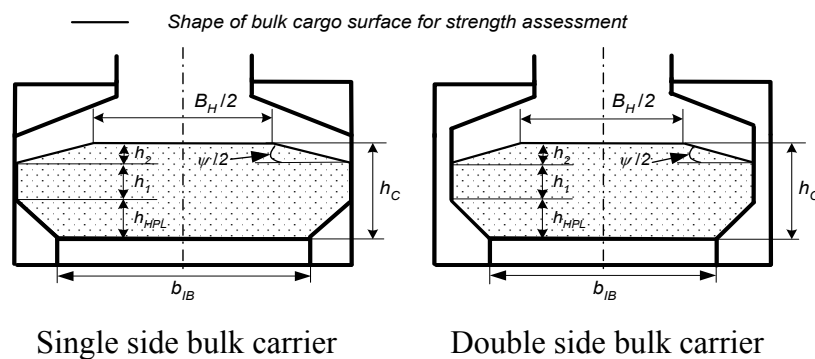
Fig. 2 Definitions of h_C , h_1 , h_2 and h_{HPL}
