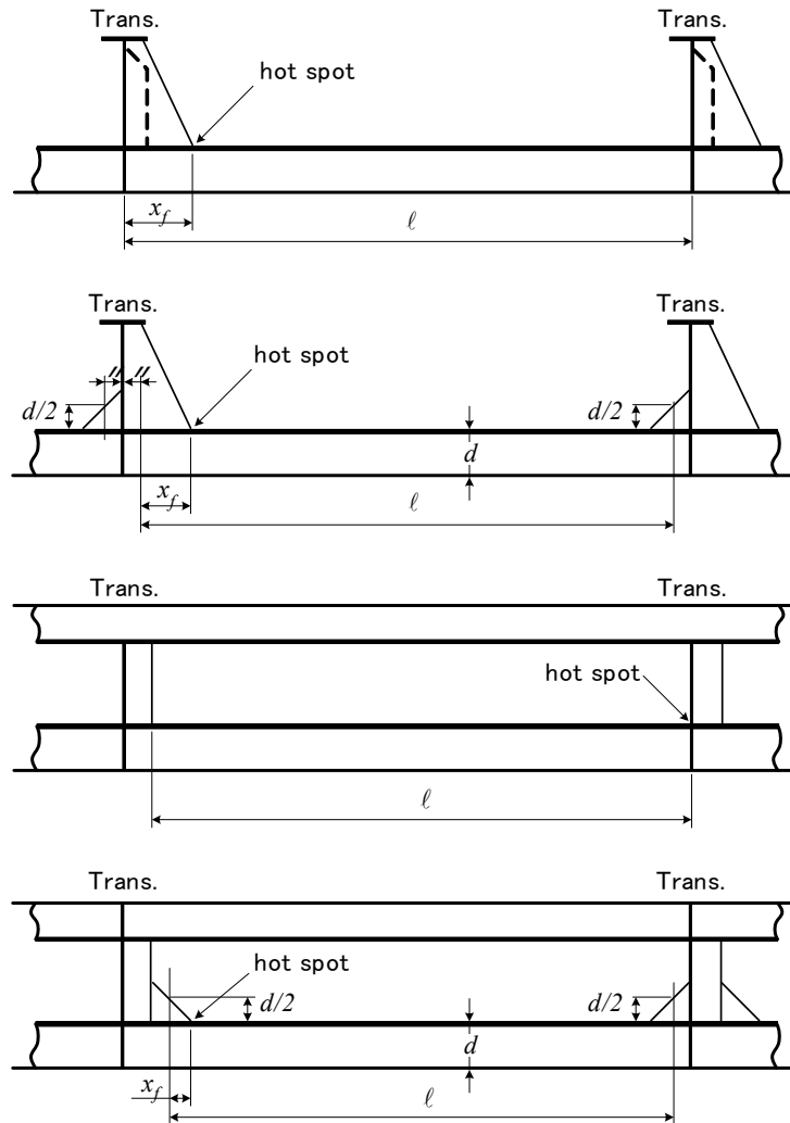
Fig. 2 Span and hot spot of longitudinal stiffeners
