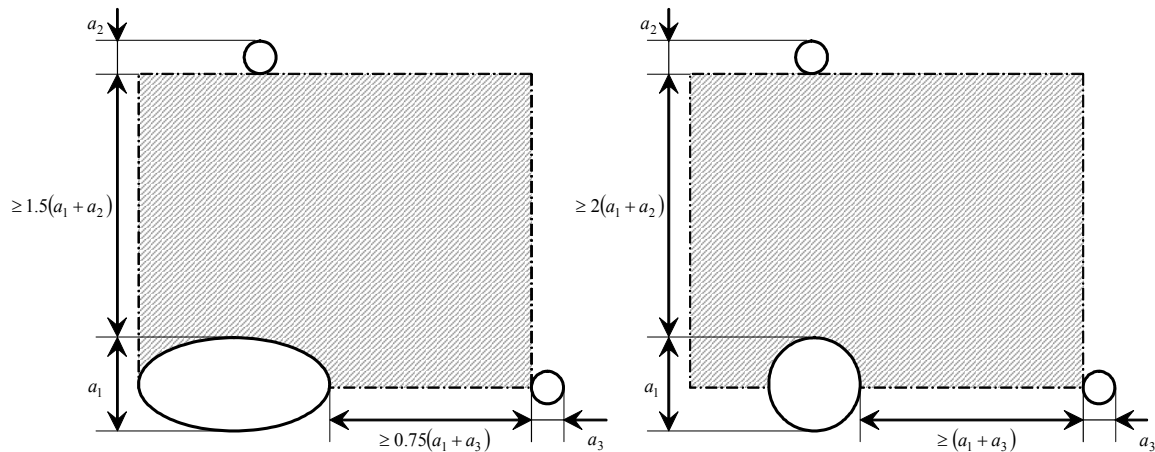
Fig. 24 Elliptical and circular openings in strength deck
