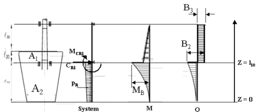
Fig. 7 Spade rudders with rudder trunks
