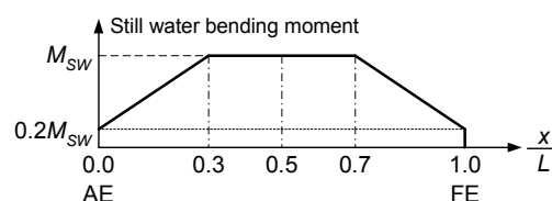
Fig. 2 Preliminary still water bending moment distribution
