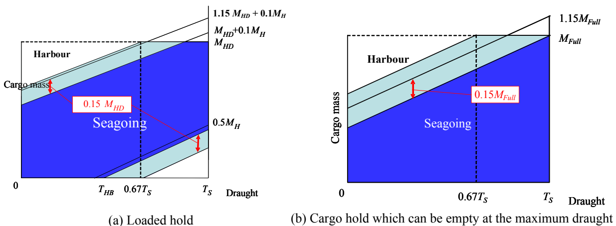
Fig. 2 Example of mass curve for BC-A ships having {No MP} assigned
