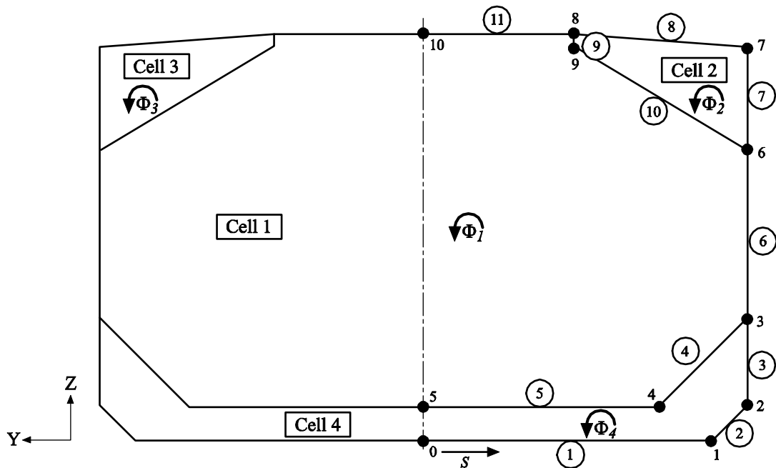
Fig. 5 Single side hull cross section
