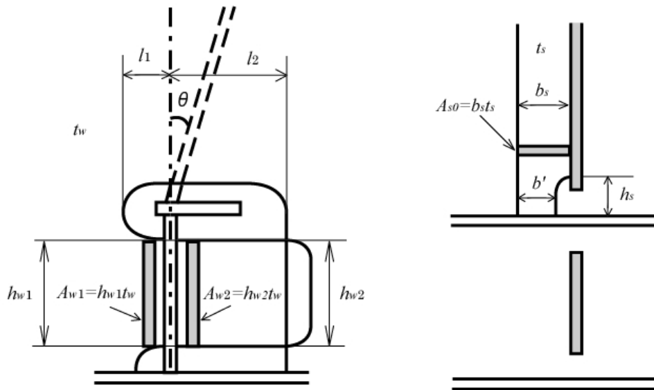
Fig. 9 Shape of the end of the web stiffener
