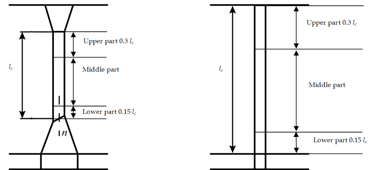
Fig. 5 Parts of Corrugation
