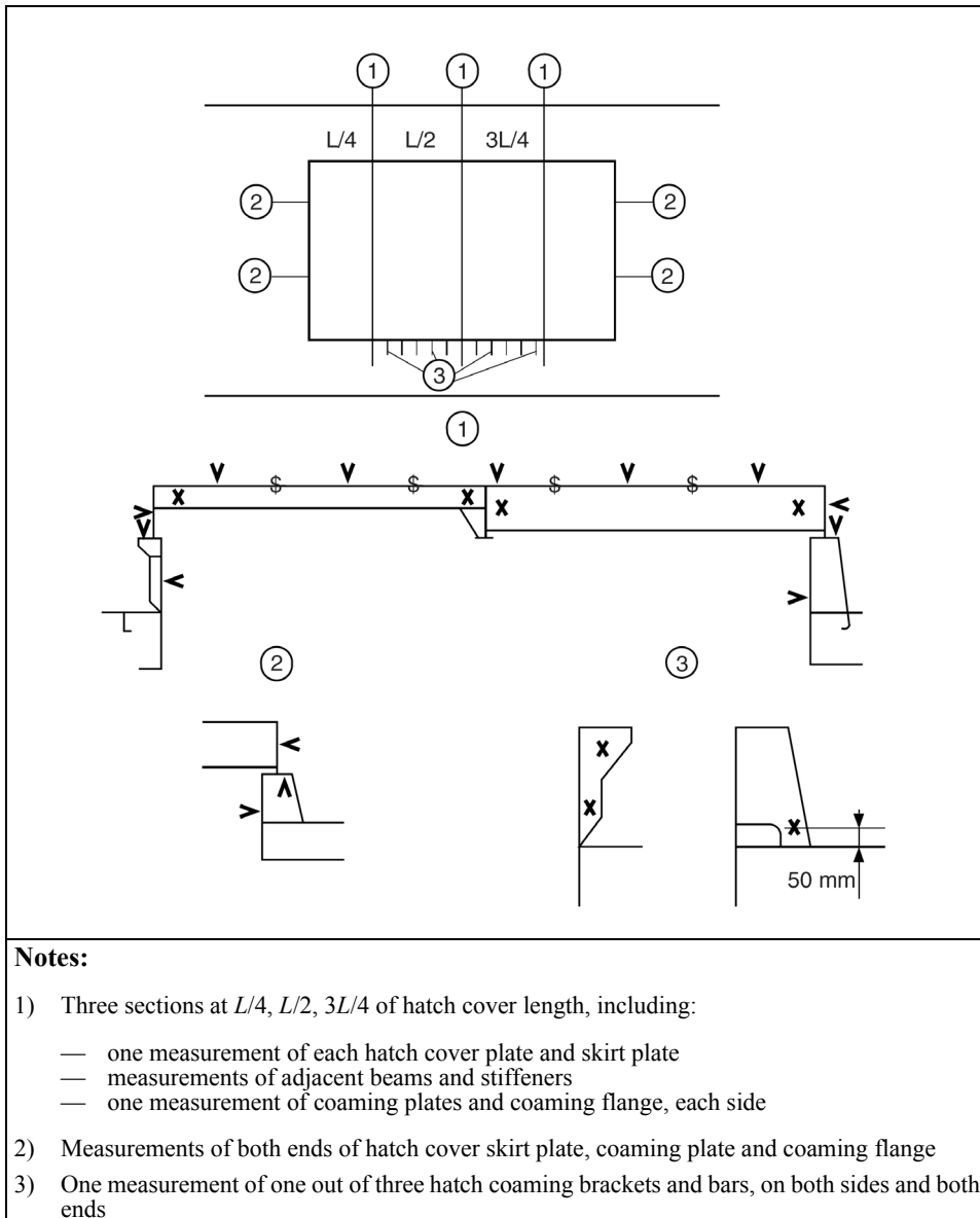
Fig. 2 Locations of measurements on hatch covers and coamings
