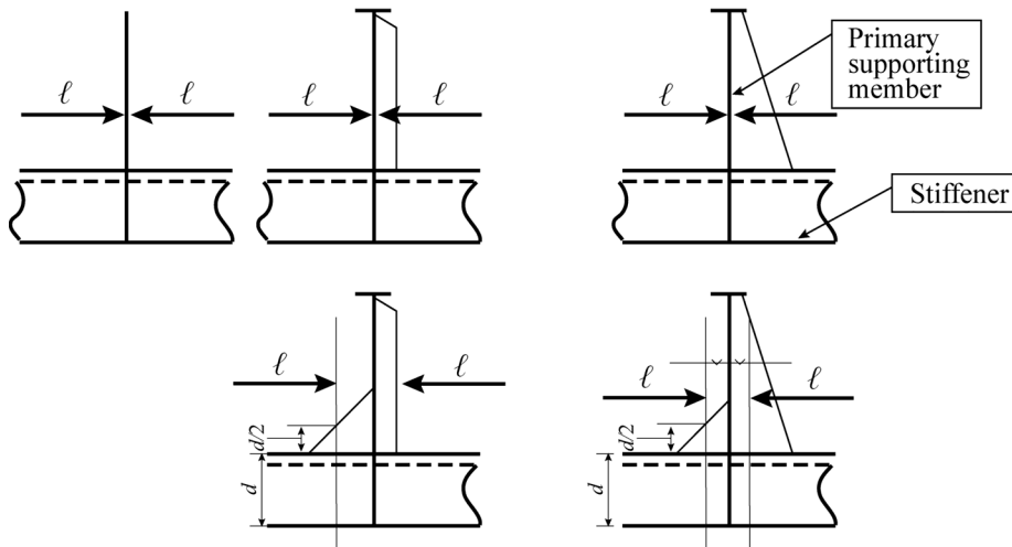
Fig. 2 Span of ordinary stiffeners
