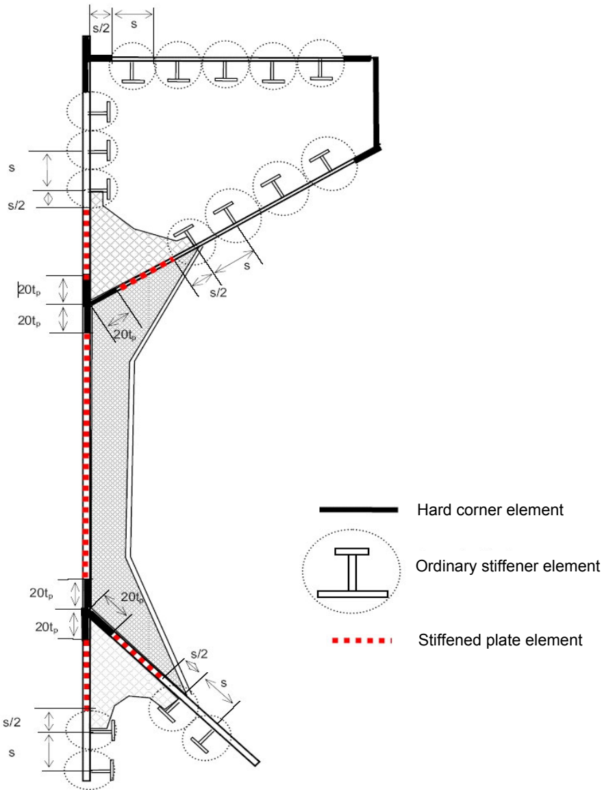
Fig. 4 Examples of the configuration of stiffened plate elements, ordinary stiffener elements and hard corner elements on a hull section
