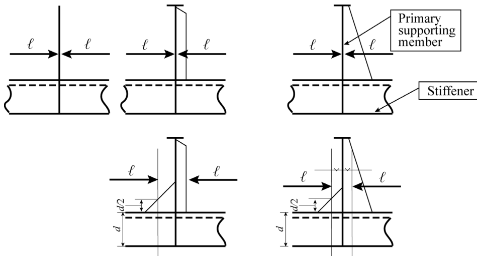
Figure 2: Span of ordinary stiffeners
