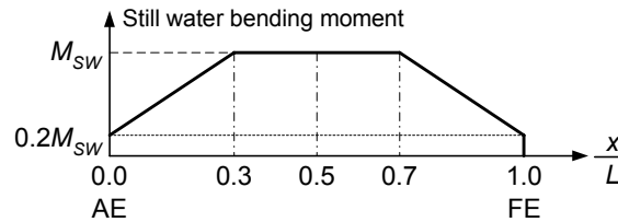
Figure 2: Preliminary still water bending moment distribution
