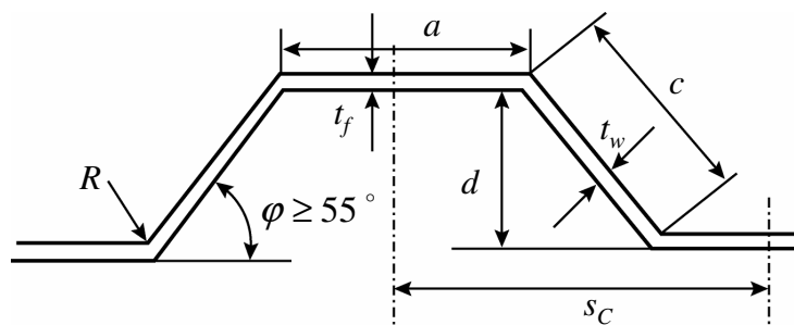
Figure 2: Corrugated bulkhead
