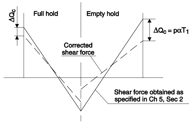
Figure 2: Shear force correction \Delta Q_C
