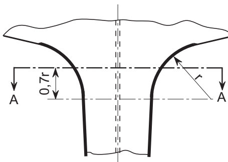
Figure 17: Transition between rudder horn and shell
