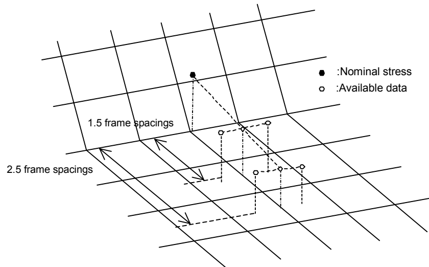
Figure 6: Definition of nominal stress at the bilge hopper knuckle part
