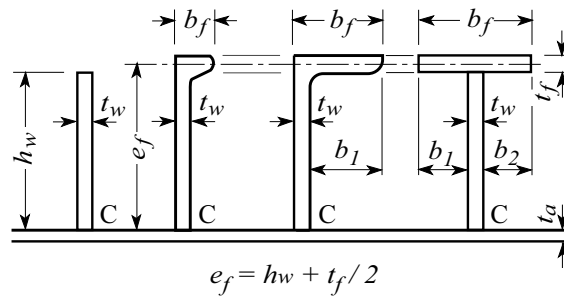
Figure 2: Dimensions of stiffeners
