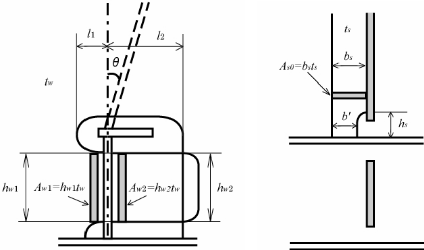
Figure 10: Definitions of geometric parameters
