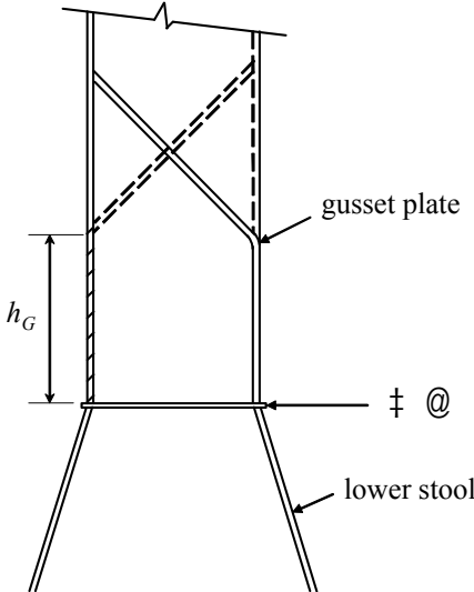
Figure 33: Symmetrical gusset/shedder plates
