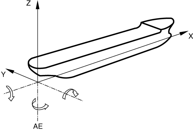
Figure 4: Reference co-ordinate system
