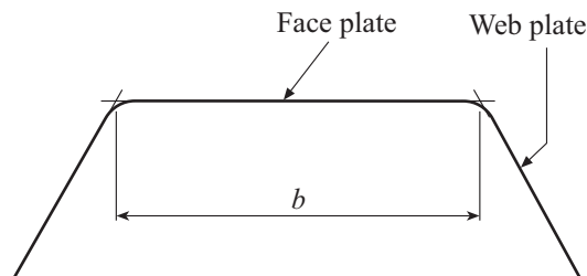
Figure 8: Measuring b of corrugated bulkheads
