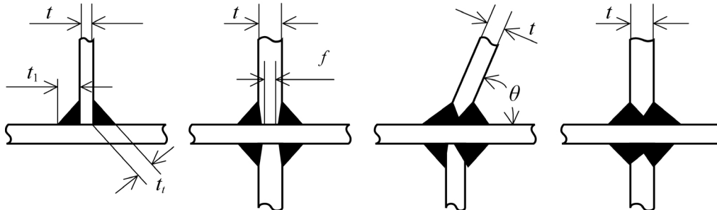
Figure 1: Tee or cross joints
