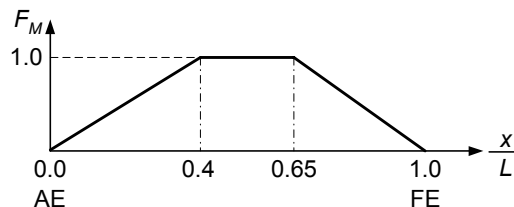
Figure 3: Distribution factor F_M
