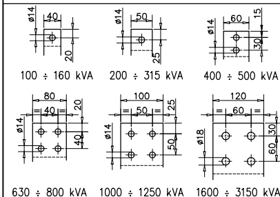
SECONDARY TERMINAL
