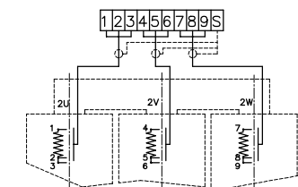
SECONDARY TERMINAL
