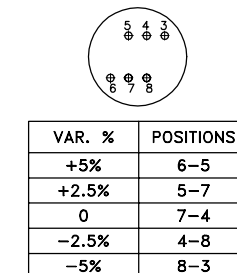
TAPS FOR PRIMARY VARIATION
