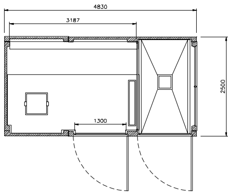
planta EHCP 4 T1D PF
