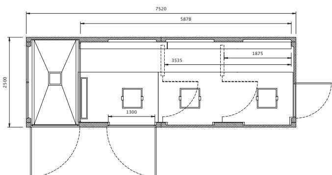
planta EHCP 8 T2D PF
