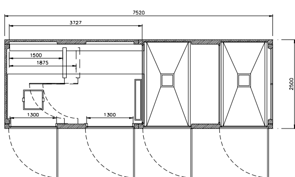
planta EHCP 8 T2D PF
