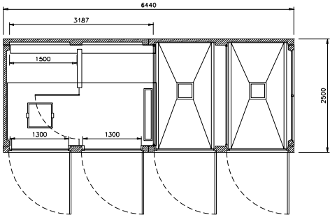
planta EHCP 6 T2D PF
