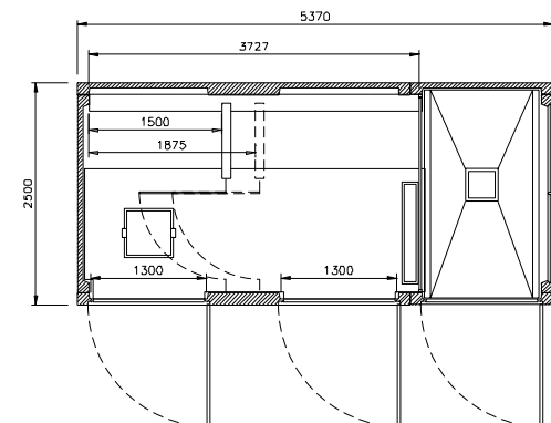
planta EHCP 5 T1D PF
