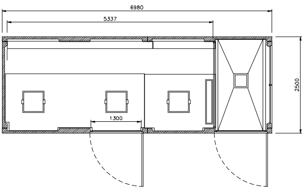
planta EHCP 7 T1D PF
