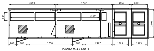
PLANTA M111 T2D PF
