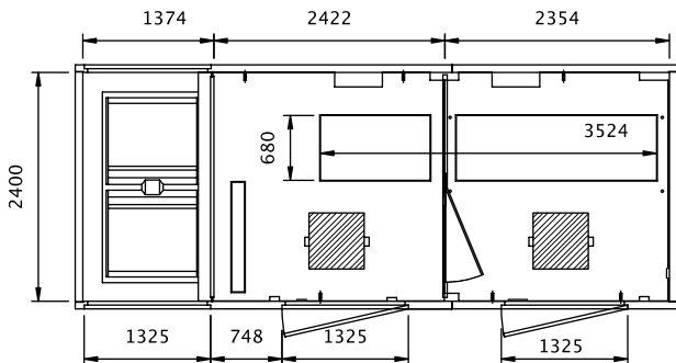
PLANTA M110 T1E PF 36
