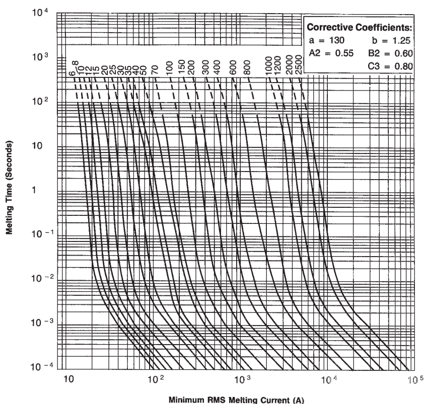
Time/Current Characteristics
