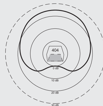
Directional diagram
