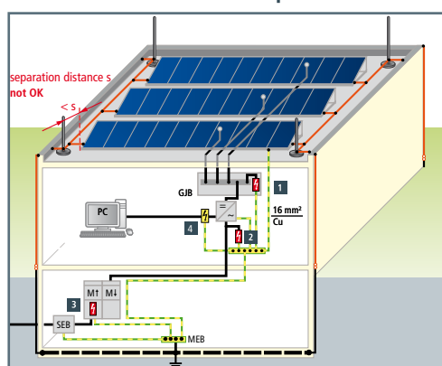
c) Building with external lightning protection and insufficient separation distance
