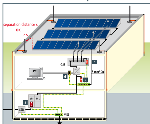
b) Building with external lightning protection and sufficient separation distance
