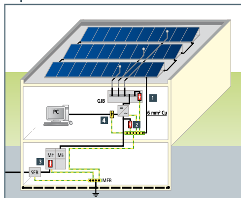
a) Building without external lightning protection
