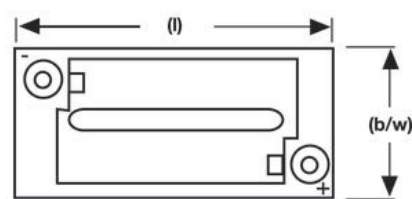
P12V1220
